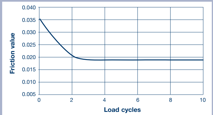
Figure 4: Friction values
